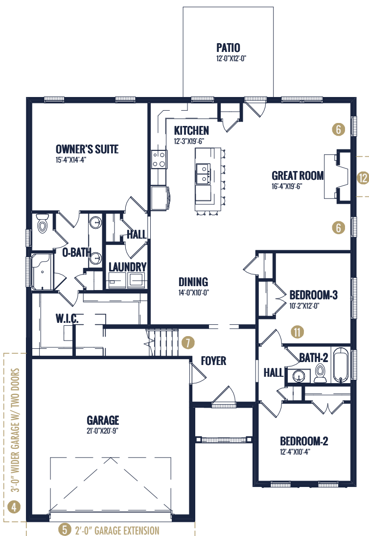
MAIN LEVEL
